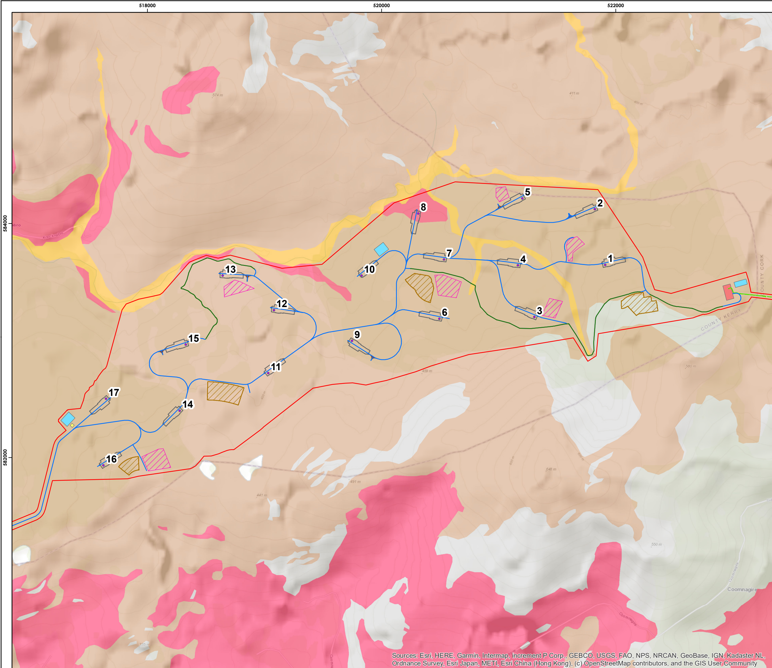
Figure10-2b Quaternary Sediments
